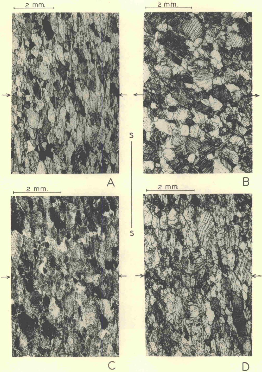
PHOTOMICROGRAPHS OF DEFORMED YULE MARBLE
